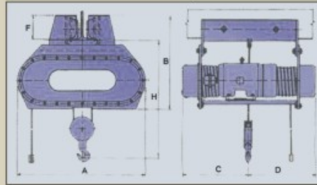
Push-Poll Trolley Hoist
