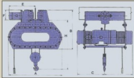
Motorized Trolley Hoist
