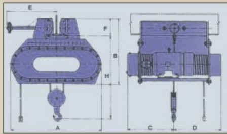
Hand Geared Trolley Hoist
