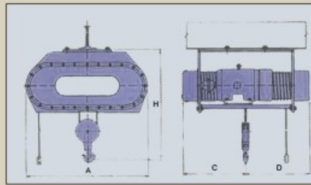
Fixed Suspension Hoist
